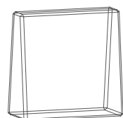
2.060.060.020.-40 60 x 60 x 20/10 mm 2.080.080.025.-40 80 x 80 x 25/12,5 mm 2.100.100.030.-40 100 x 100 x 30/15 mm
